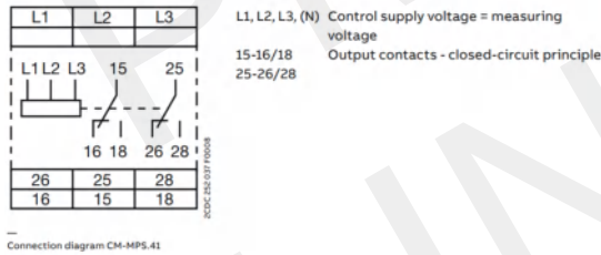
Connection diagram CM-MPS.41
